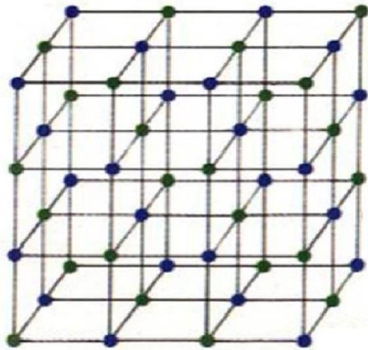
Crystalline three-dimensional-lattice-structure
